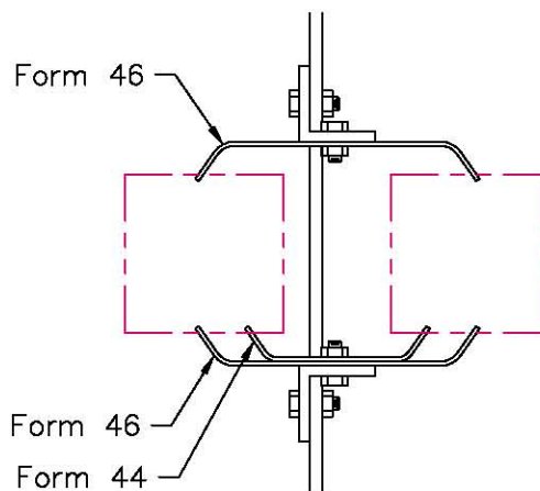
3-Point Contact Assembly
