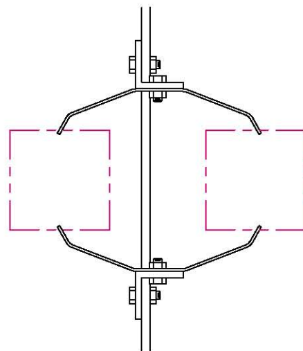
2-Point Contact Assembly
