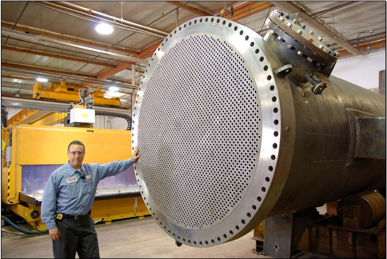
72" DIAMETER TITANIUM HEAT EXCHANGERS WITH EXPLOSION CLAD TUBESHEETS FOR THE MANUFACTURE FOR PTA
